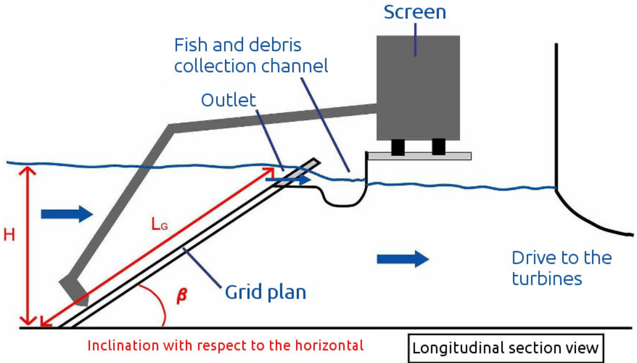
Figure 9.3: Inclined trashrack
